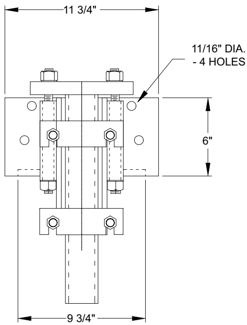
Model TAB-150-UB Utility Bracket Details
