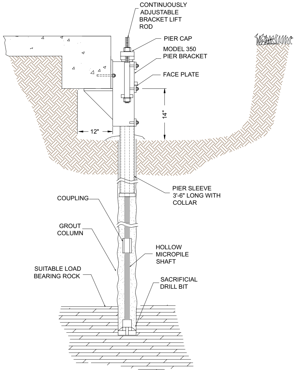
Model 350-MP2 – Typical Micro Pile Application Drawing
