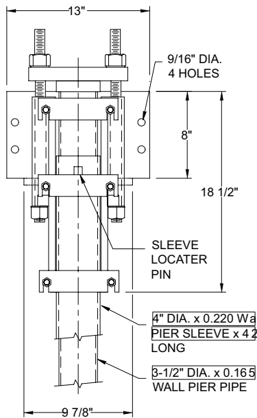
Model 350-MP2 Micro Pile Bracket Details
