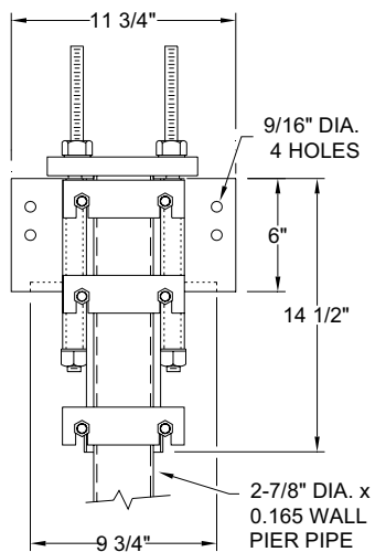
Model 300 Utility Bracket Details
