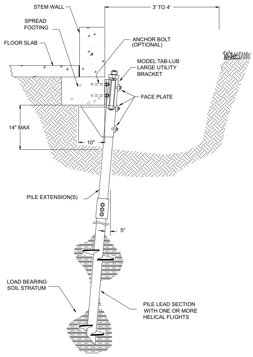
Model TAB-288-LUB Large Utility Bracket Application Drawing
