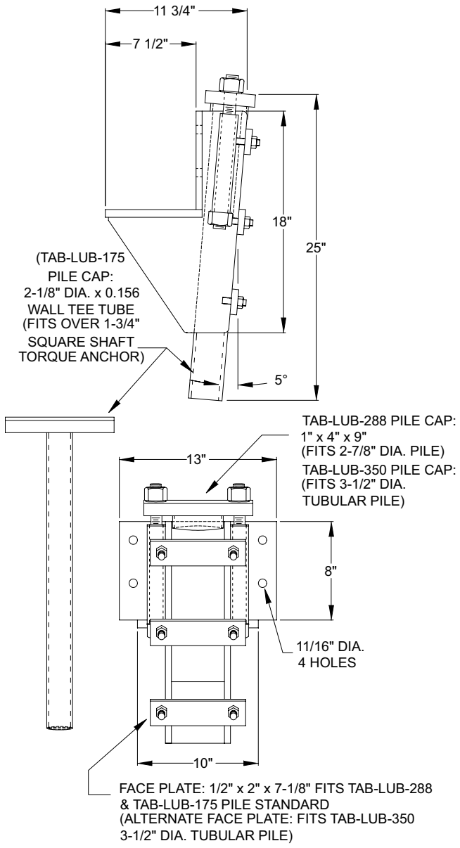
Model TAB-LUB Large Utility Bracket Details
